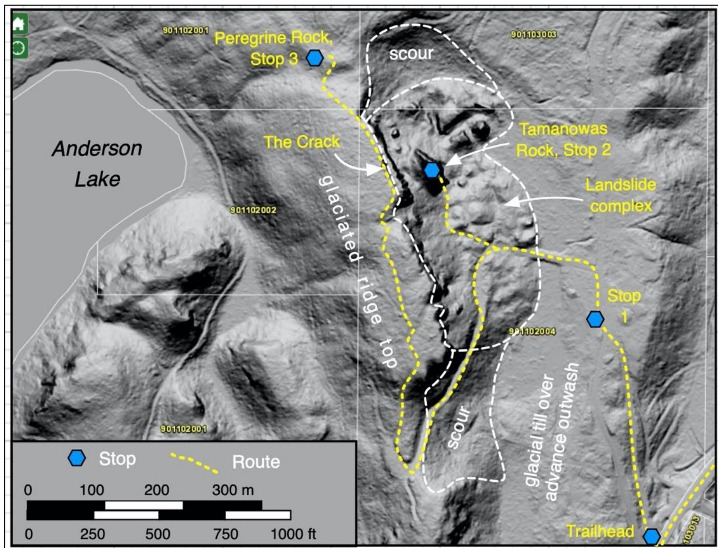
Figure 9. Landslide debris at and around Tamanowas Rock. The route is shown as yellow dotted line. Areas of scour are based solely on morphology. Fine white lines and small yellow numbers are parcel boundaries and identifiers from https://gisweb.jeffcowa.us/LandRecords/ .
