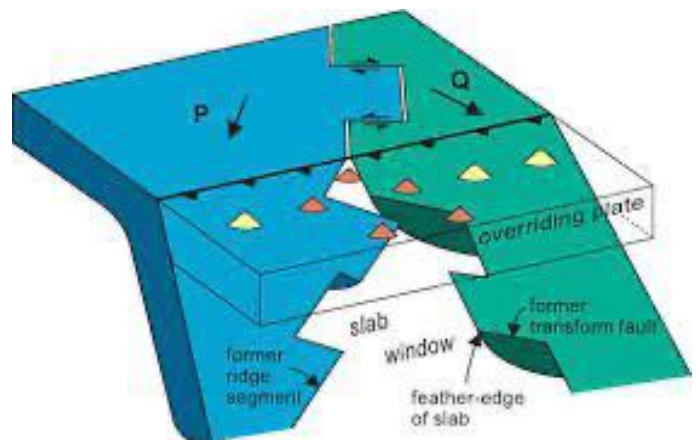
Figure 7. Diagram of a slab window forming where an oceanic spreading ridge is being subducted and torn apart. Hot mantle rising through the slab window (gap in the slab) drives the subducting slab to melt at its edges, producing adakite magmas (the orange volcano symbols). P and Q indicate plate movement vectors. From Thorkelson and Breitsprecher (2004).
