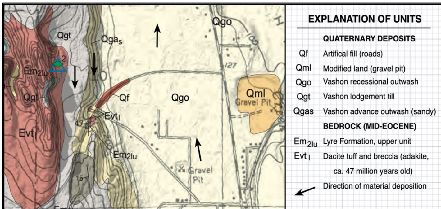
Figure 5. Geologic map of the area around Tamanowas Rock (about the same area as in Fig. 1). The gravel pit (unit Qml) is the location of HJ Carroll County Park (starting point for this trip). Mapping and explanation of units from Schasse and Slaughter (2005). Blue triangle and green diamond are sampling locations for dating the rock.
