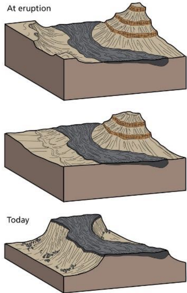
Figure 8. Diagram showing how a resistant rock (lava flow) can lead to inverted topography. (National Park Service)
