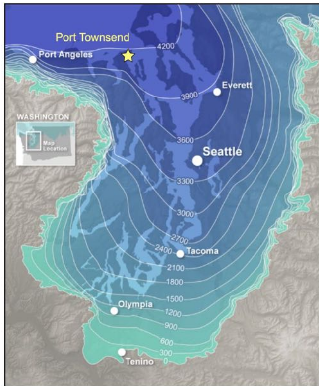
Figure 2. Schematic map of ice thickness in feet for the Puget lobe at its maximum extent, about 17,000 years ago. (WADNR, 2022).
