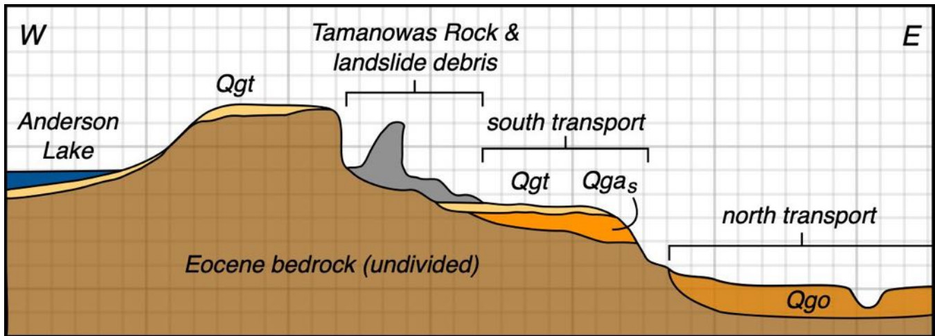
Figure 10. Diagrammatic cross-section of the Tamanowas Rock area. Geology is based on Figure 5; see the explanation of that figure for definition of geologic unit symbols. All subsurface contacts are interpretations with no depth control. Note the south-transported units are early glacial advance outwash and till, whereas the more deeply channelized meltwater flowed to the north, leaving recessional outwash deposits. Anderson Lake sits in a glacially excavated basin. Geologic relations are our interpretation based on mapping of Schasse and Slaughter (2005).
